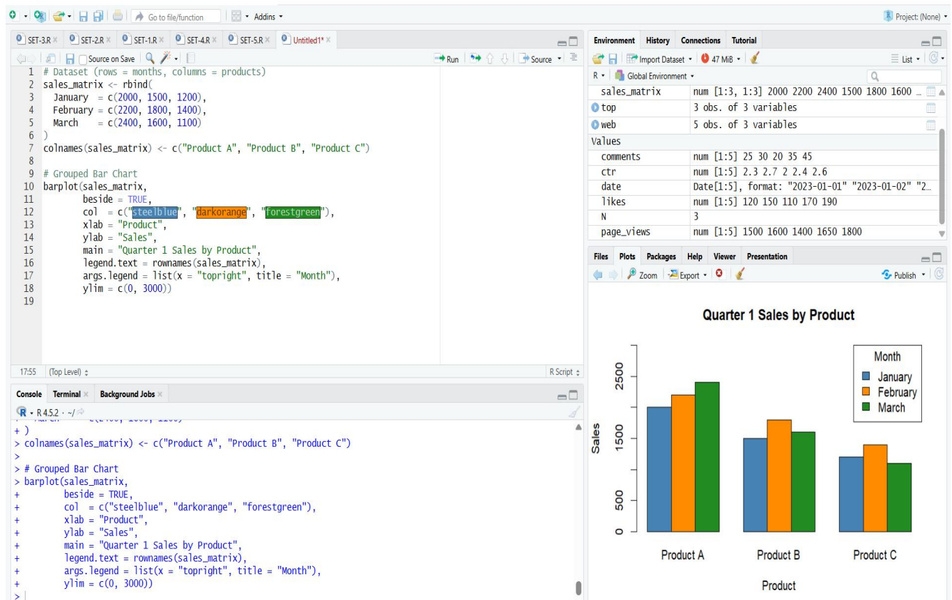
Output 1: Quarter 1 Sales by Product (Grouped Bar Chart)
